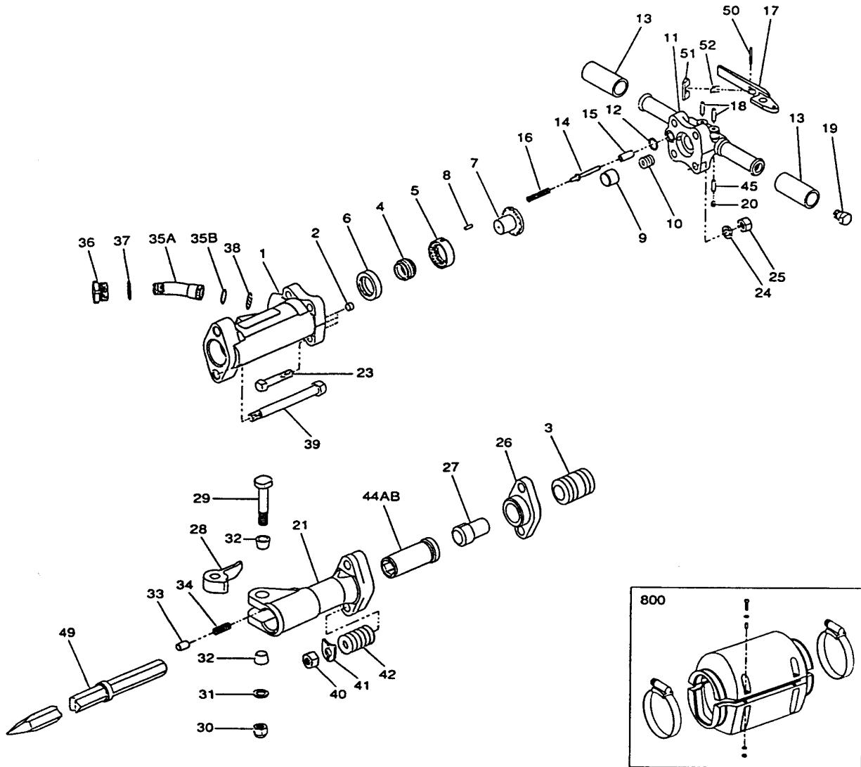
Latch Kit
